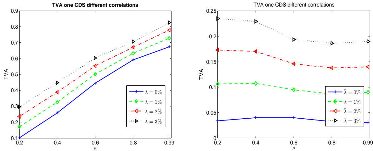
Figure 1. Left : TVA on one CDS as a function of the correlation parameter \rho and for different bank credit spreads \bar{\lambda} , in a DGC model with three names: the bank, its counterparty and the reference credit name of the CDS. Right : Analog results in a fake DGC model without wrong-way-risk.
