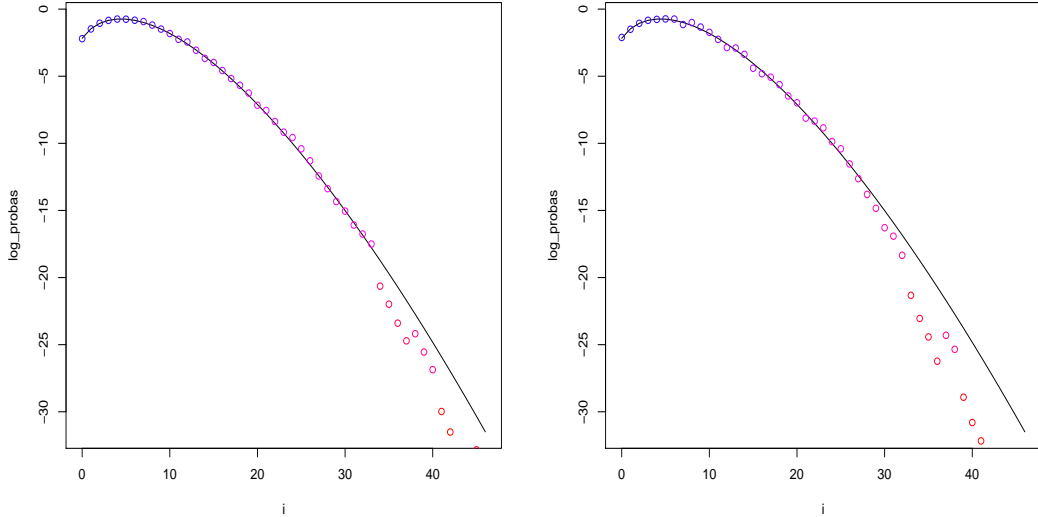
FIGURE 6. IPS Values , d = 5 . Left panel : m = 20000 ; Right panel : m = 5000 .
