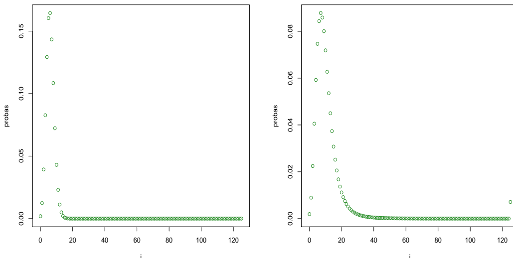
FIGURE 7. 5y loss distributions. Left panel: Independent obligors ( a = 0.01, b = 0 ); Right panel: Extreme contagion ( a = 0.01, b = 13 ).
