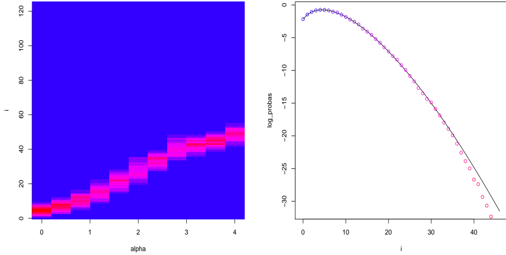
FIGURE 3. IPS losses (left) and log-probabilities (right). We used d = 1 and m = 10^5 .
