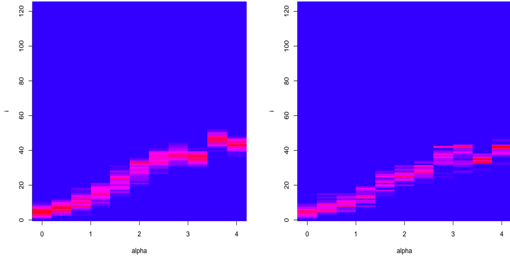
FIGURE 5. IPS Losses , d = 5 . Left panel : m = 20000 ; Right panel : m = 5000 .
