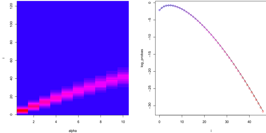
FIGURE 2. IS losses (left) and log-probabilities (right). d = 5 and m = 5000 .
