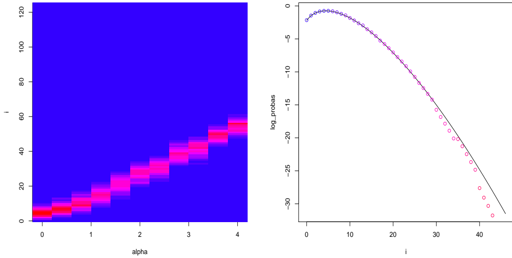
FIGURE 4. IPS losses and log-probabilities. We used d = 5 and m = 10^5 .
