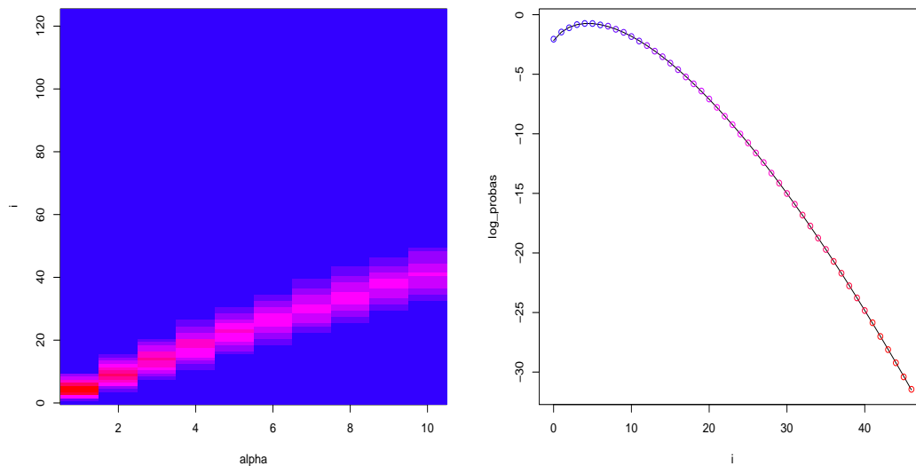
FIGURE 1. IS losses as function of alpha (left) and log-probability estimates (dots) superimposed on the exact probabilities (right). We used d = 1 and m = 5000 .
