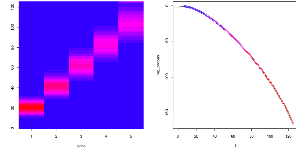
FIGURE 8. IS losses and log-probabilities for independent obligors ( a = 0.01, b = 0, m = 10000 ).
