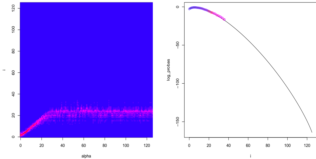
FIGURE 11. IPS losses and log-probabilities in the case of independent obligors ( a = 0.01, b = 0, m = 10000 ).
