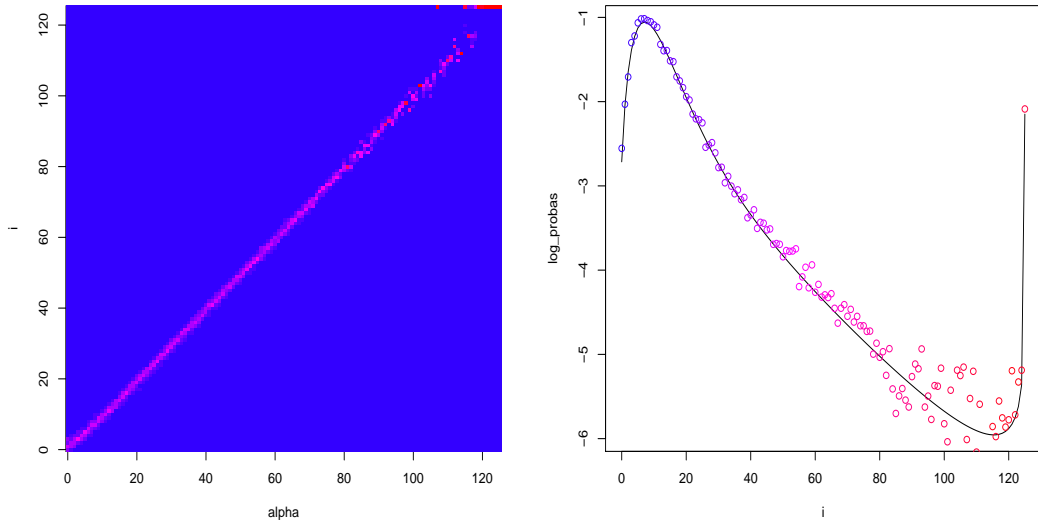
FIGURE 10. IPS losses and log-probabilities in the case of extreme contagion ( a = 0.01, b = 13, m = 10000 ).
