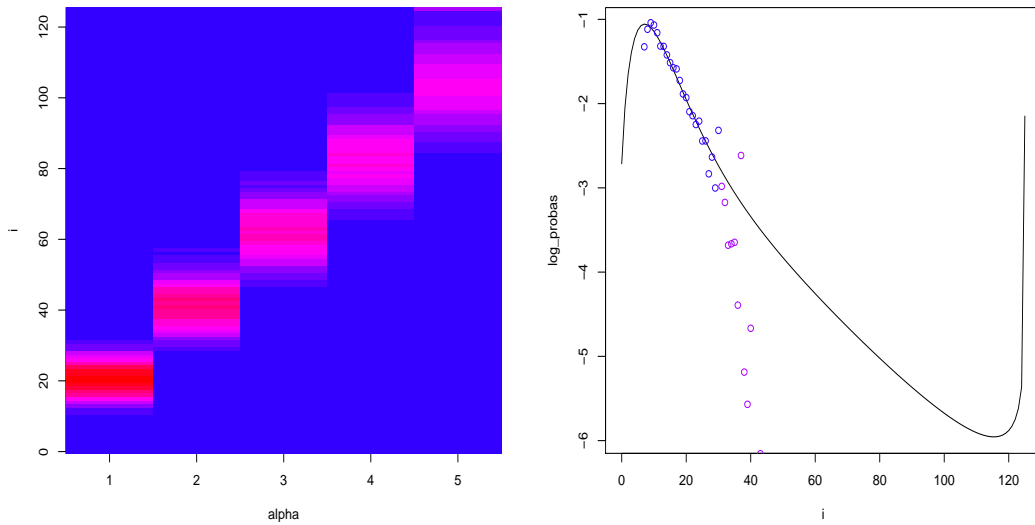
FIGURE 9. IS losses and log-probabilities in the case of extreme contagion ( a = 0.01, b = 13, m = 10000 ).
